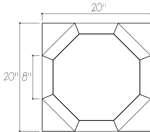
Plan/ Top View
